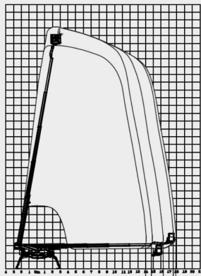
RUTHMANN BLUELIFT ST 31
